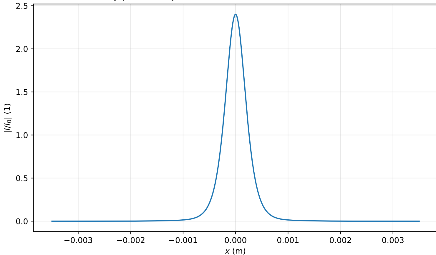
Intensity profile I(x, y = 0, z = 2.548m)/I_0 , P_{in}=1.0P_{cr} , artificial time
